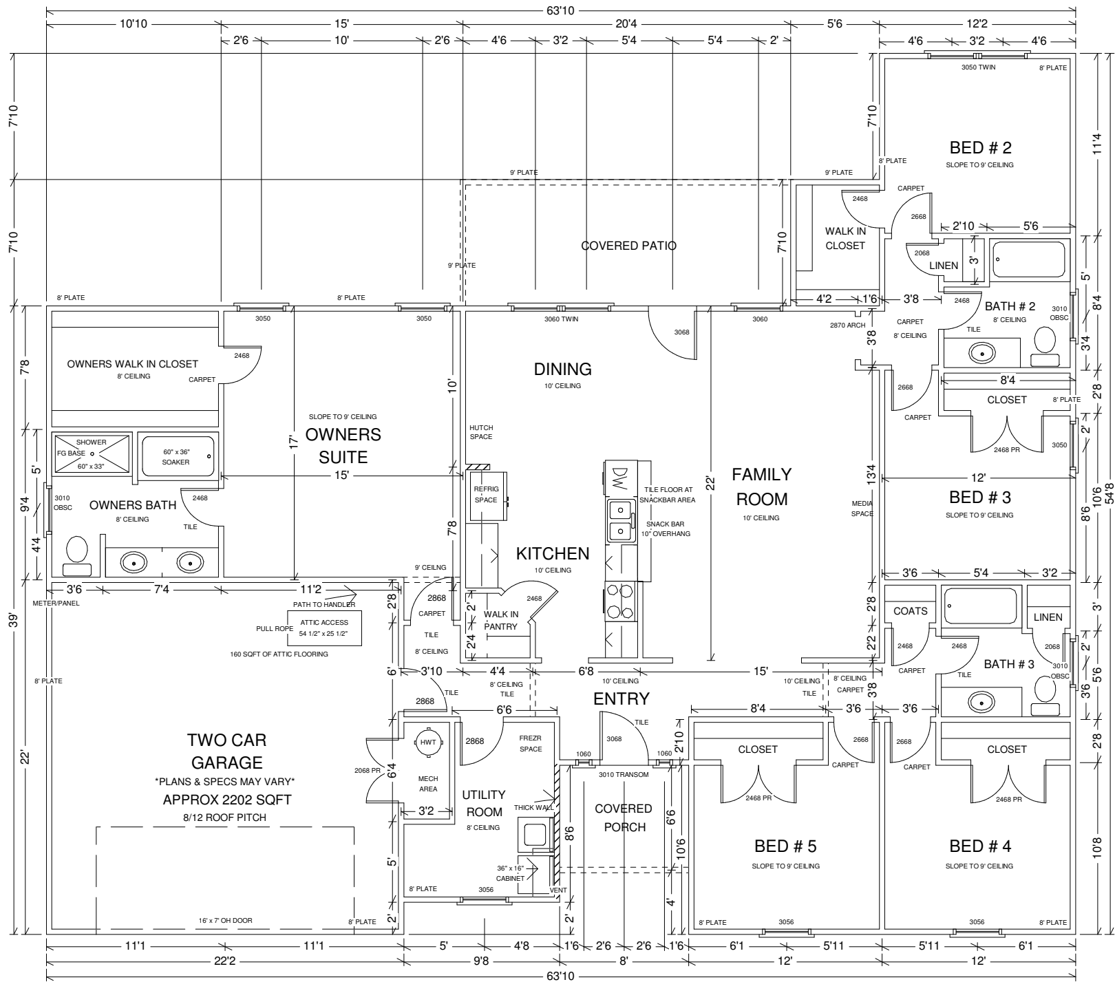
PRESCOTT PLAN
