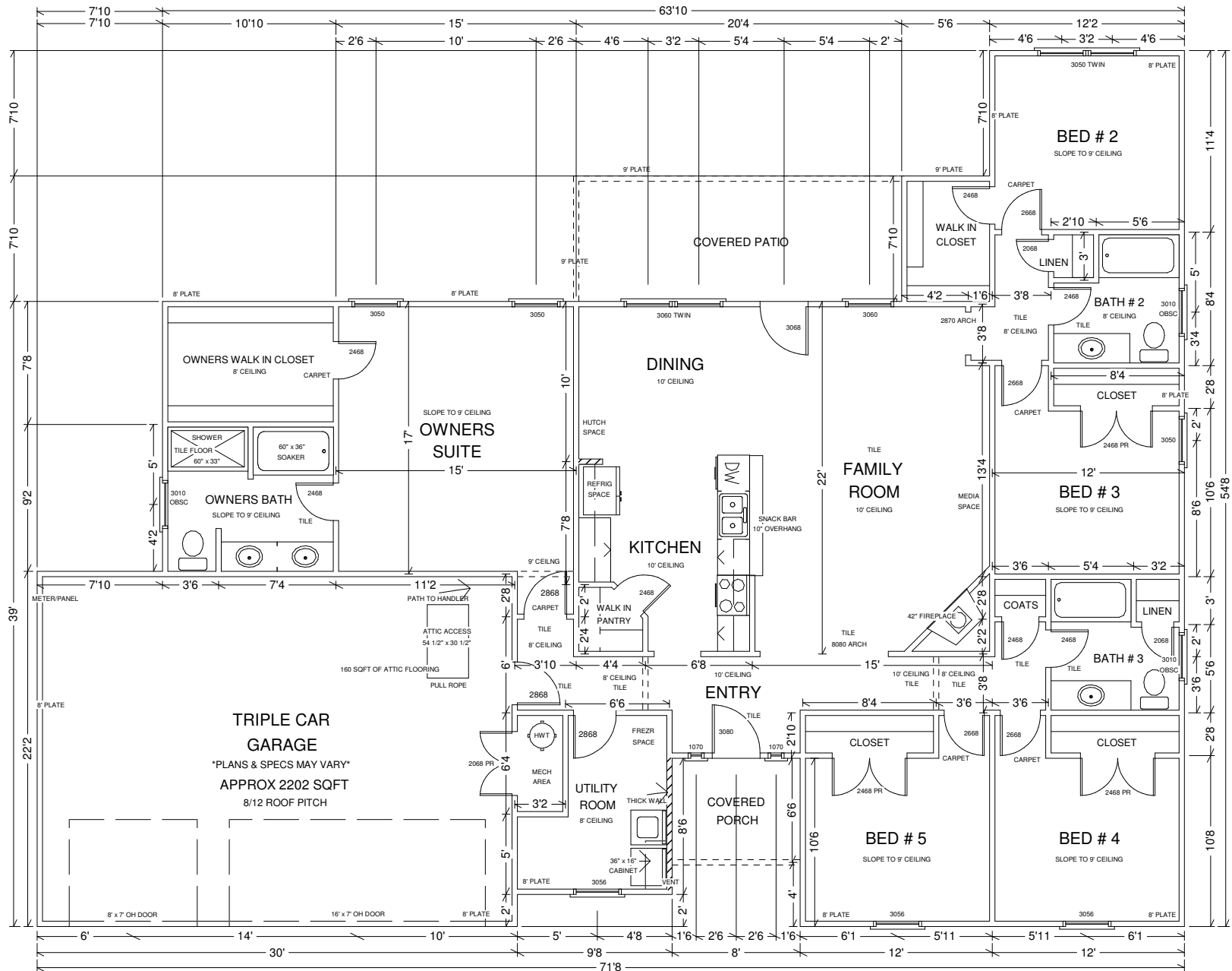
CITATION PLAN
